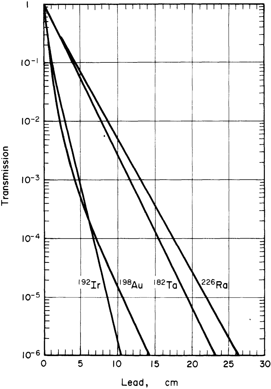
Fig. C13. Broad-beam transmission of gamma rays from various radionuclides through lead, density 11 350 kg m -3 .
