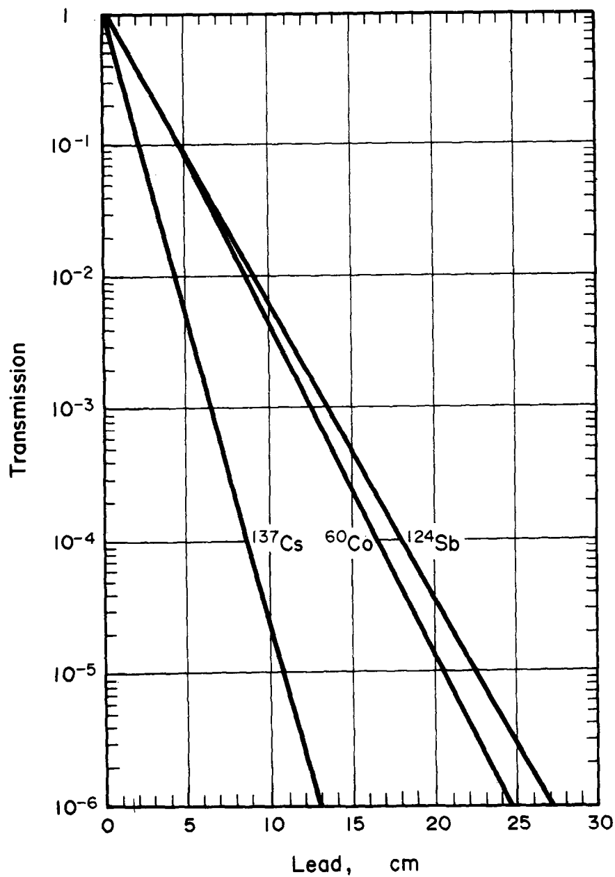
Fig. C12. Broad-beam transmission of gamma rays from various radionuclides through lead, density 11\,350\text{ kg m}^{-3} .
