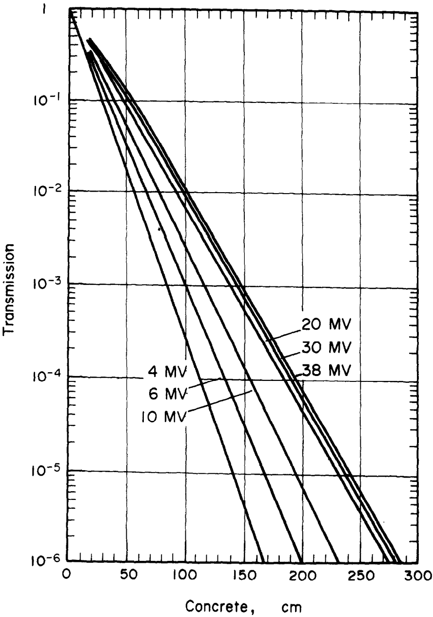
Fig. C3. Broad-beam transmission of X rays through concrete, density 2350 \text{ kg m}^{-3} . 4 MV: linear accelerator; 1 mm gold target followed by 20 mm aluminium beam flattener. 6-38 MV: Betatron; target and filtration not stated. The 38 MV curve may be used up to 200 MV (Miller and Kennedy, 1956).
